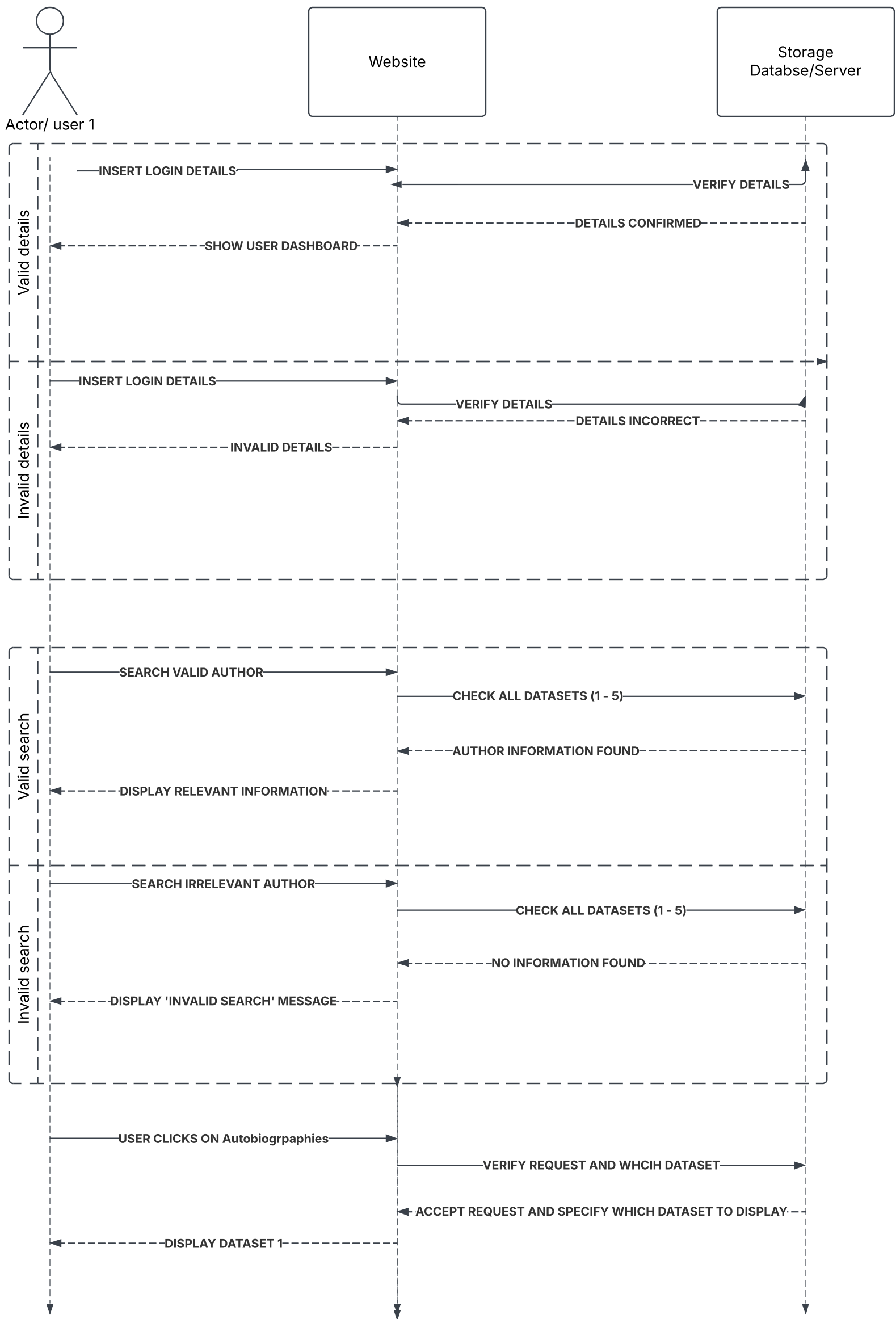
UML Sequence diagram
